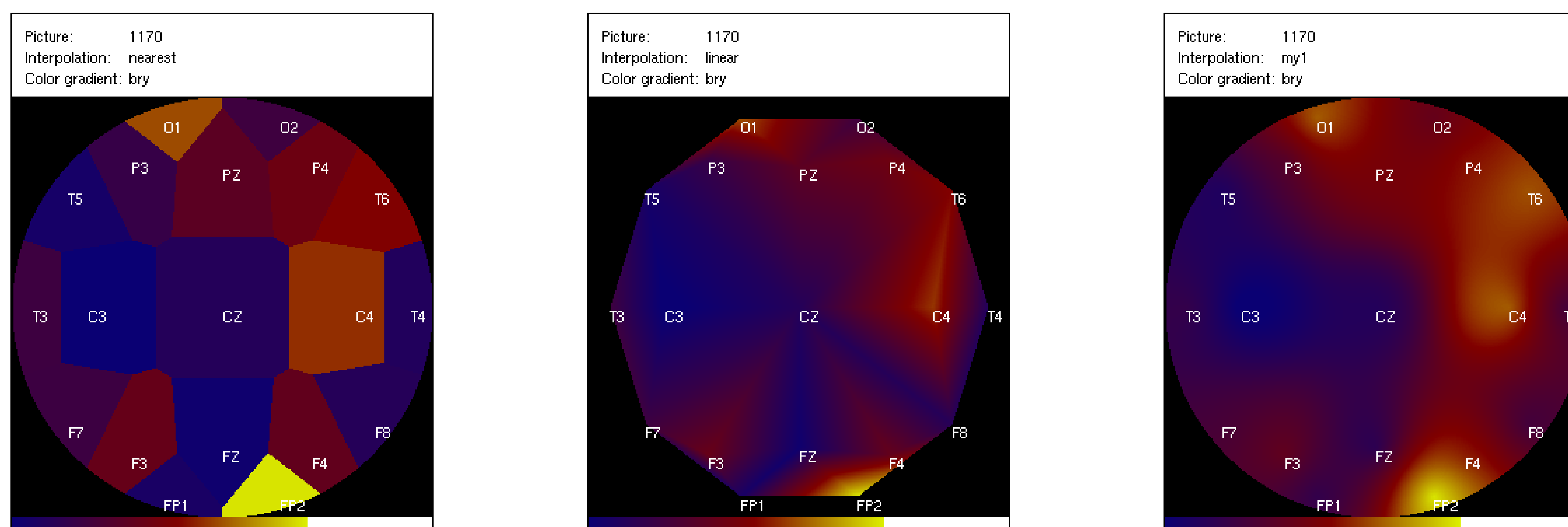
Figure 2: Output from distributed computing engine in Python - Different interpolation methods (Nearest neighbor, Linear, Weighted distance)
